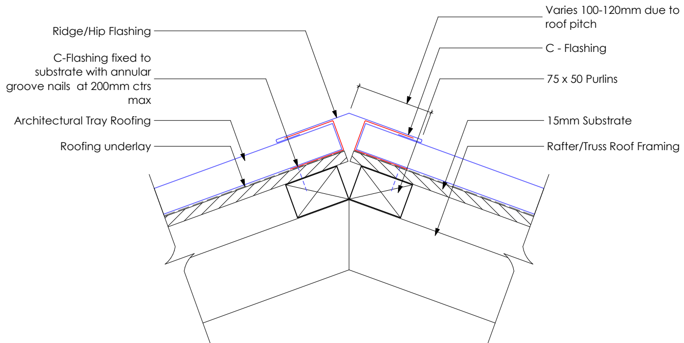
Ridge & Hip Detail Architectural Tray Scale 1:5 The Architectural Roofing Company info@trayroofing.co.nz
