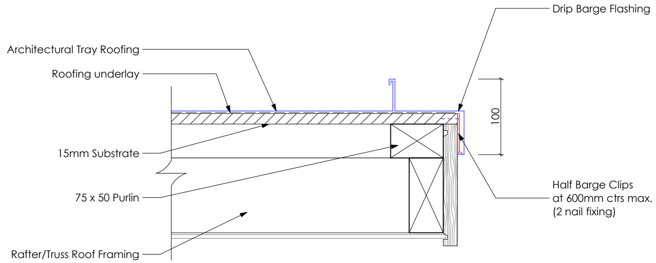
Gable End Side Drip Barge Detail Architectural Tray Scale 1:5 The Architectural Roofing Company info@trayroofing.co.nz
